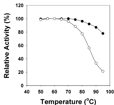
FIGURE 4: Determination of the thermal stability of SLeuRS \alpha\beta . SLeuRS \alpha\beta (40 \mu g/mL) in 50 mM potassium phosphate buffer, pH 6.8, containing 400 \mu g/mL BSA was incubated at various temperatures (50–95 °C) for 10 min. Then, the aminoacylation activity of SLeuRS \alpha\beta (filled circles) was assayed at 37 °C after dilution of the reaction mixture with cold 50 mM potassium phosphate buffer, pH 7.5, and compared with that of A. aeolicus \alpha\beta -LeuRS [open circles (6)].
